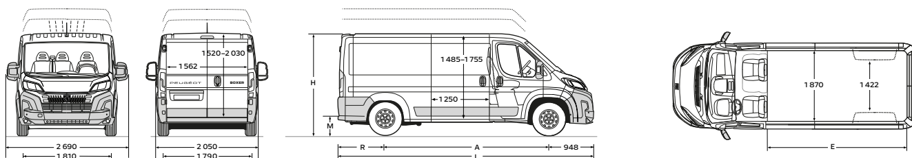
X250 Boxer Furgon
